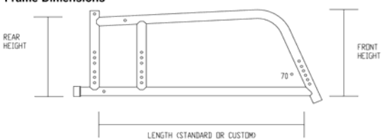
Frame Dimensions
